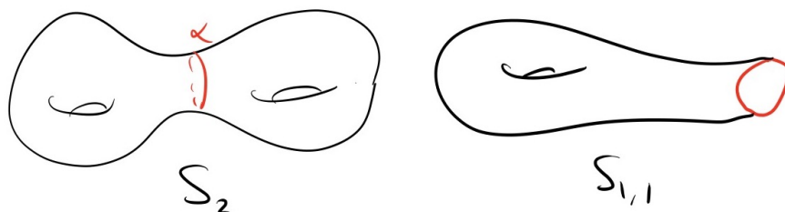
FIGURE 1. The surfaces in problem 6.
