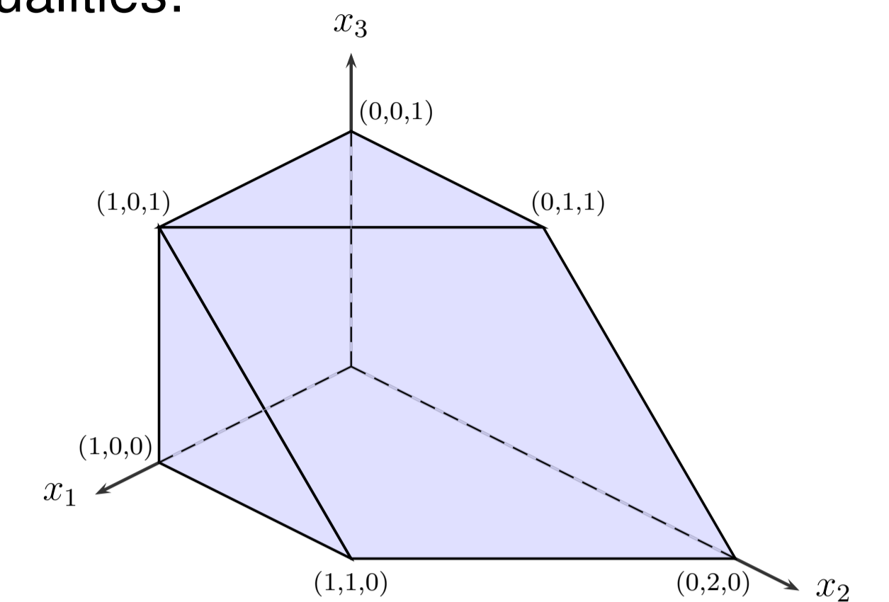
Figure 2. The Okounkov body of \mathcal{O}_{\mathbf{P}(T_{\mathbb{P}^2})}(1) .
